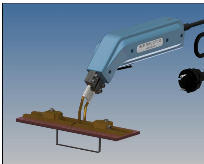
Profile cut adapter with HSGM-Styro-Cut-230 (HSGM-Styro-Cut 230 and cutting band not included in scope of delivery!)
